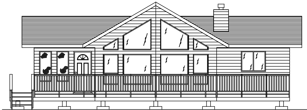
FRONT ELEVATION
